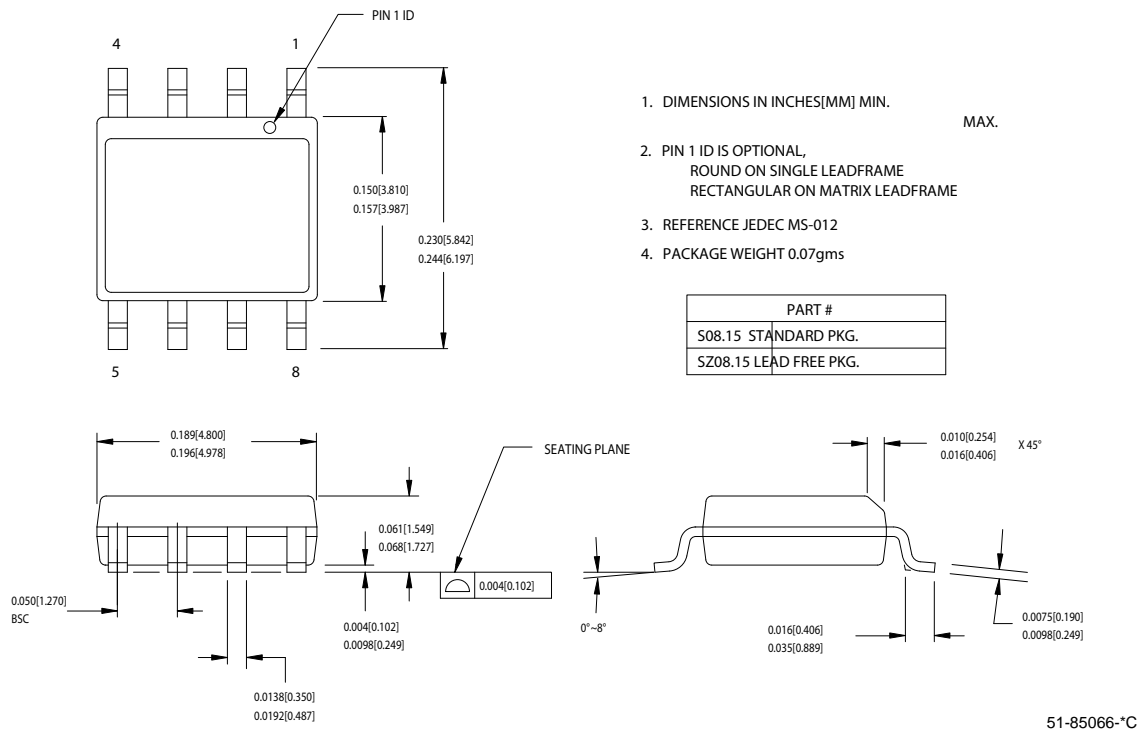
Figure 6. 8-Lead (150-Mil) SOIC S8
